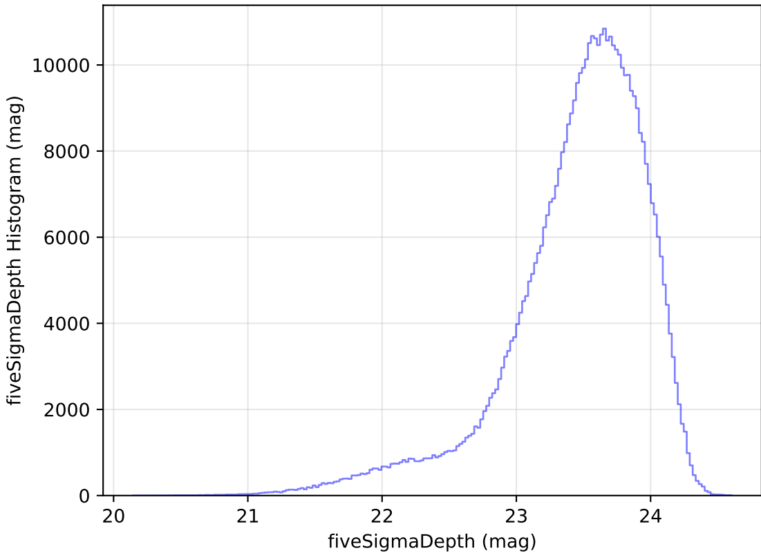
too_elab_r16_d2_gz_v3.4_10yrs i: fiveSigmaDepth Histogram
