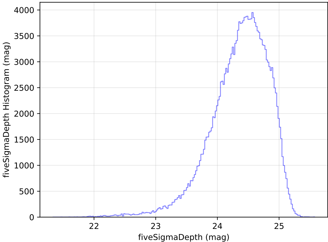
too_elab_r16_d2_gz_v3.4_10yrs g: fiveSigmaDepth Histogram
