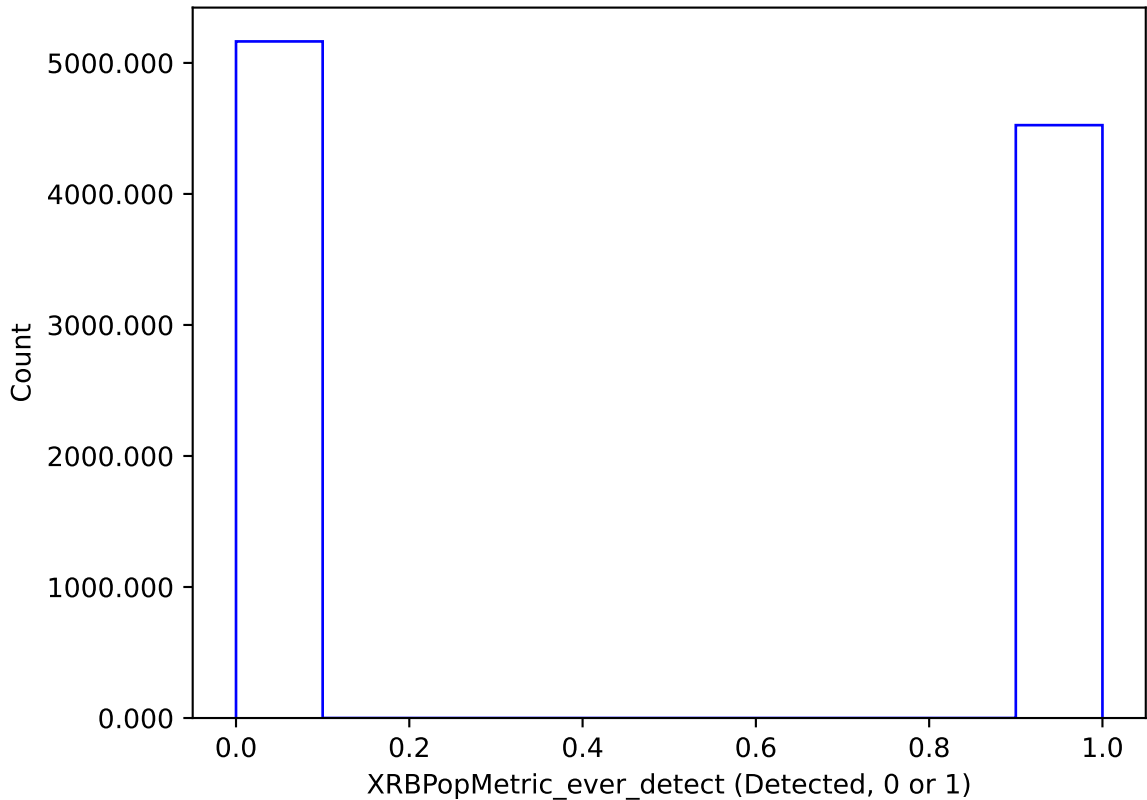
too_elab_r16_d2_gz_v3.4_10yrs : XRBPoMetric_ever_detect
