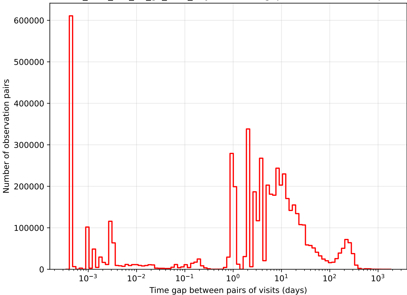
too_elab_r16_d2_gz_v3.4_10yrs i band: Tgaps observationStartMJD
