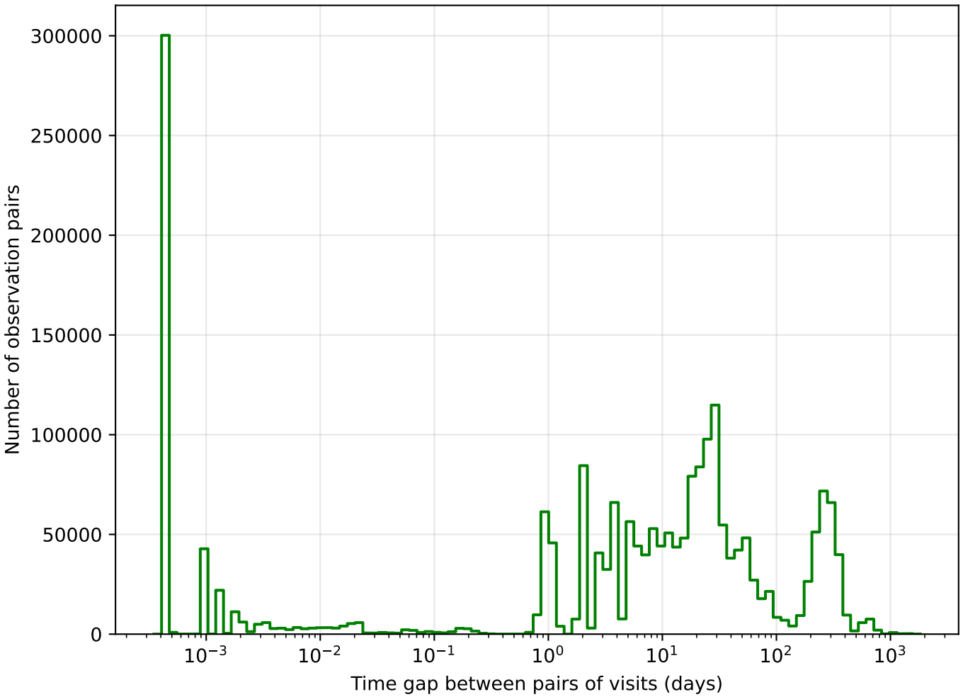
too_elab_r16_d2_gz_v3.4_10yrs g band: Tgaps observationStartMJD
