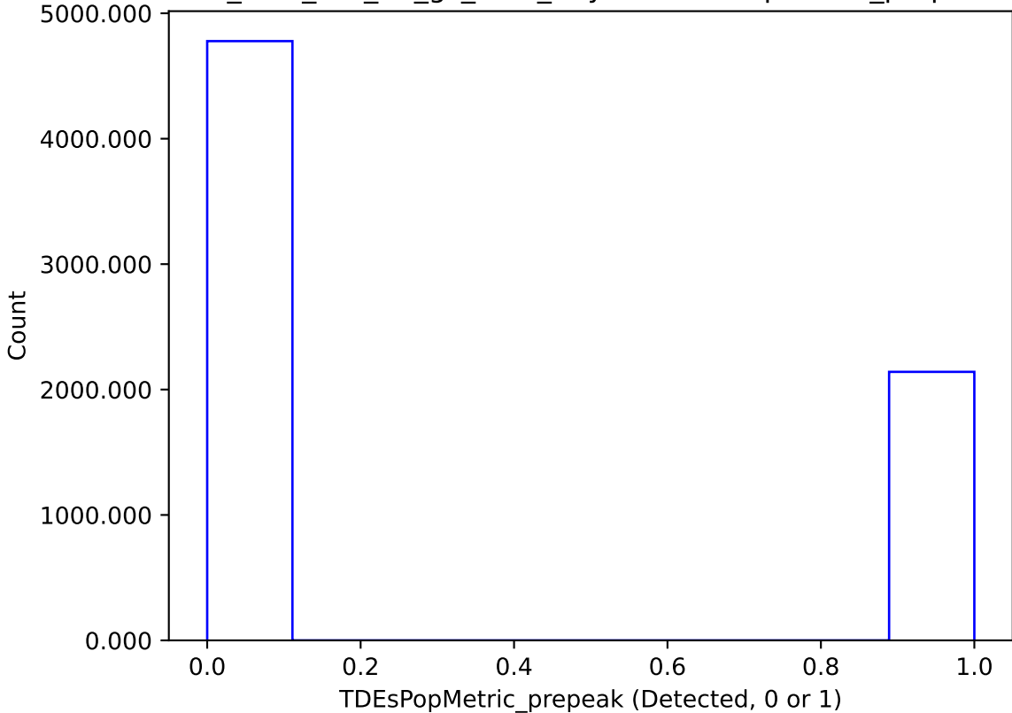
too_elab_r16_d2_gz_v3.4_10yrs : TDEsPopMetric_prepeak
