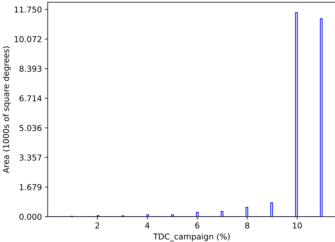
too_elab_r16_d2_gz_v3.4_10yrs : TDC_campaign
