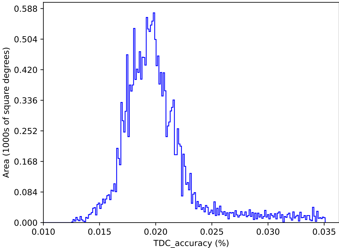
too_elab_r16_d2_gz_v3.4_10yrs : TDC_accuracy
