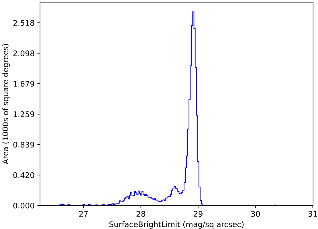
too_elab_r16_d2_gz_v3.4_10yrs u: SurfaceBrightLimit
