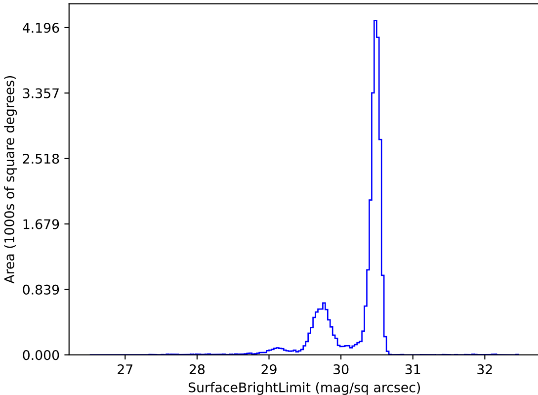
too_elab_r16_d2_gz_v3.4_10yrs r: SurfaceBrightLimit
