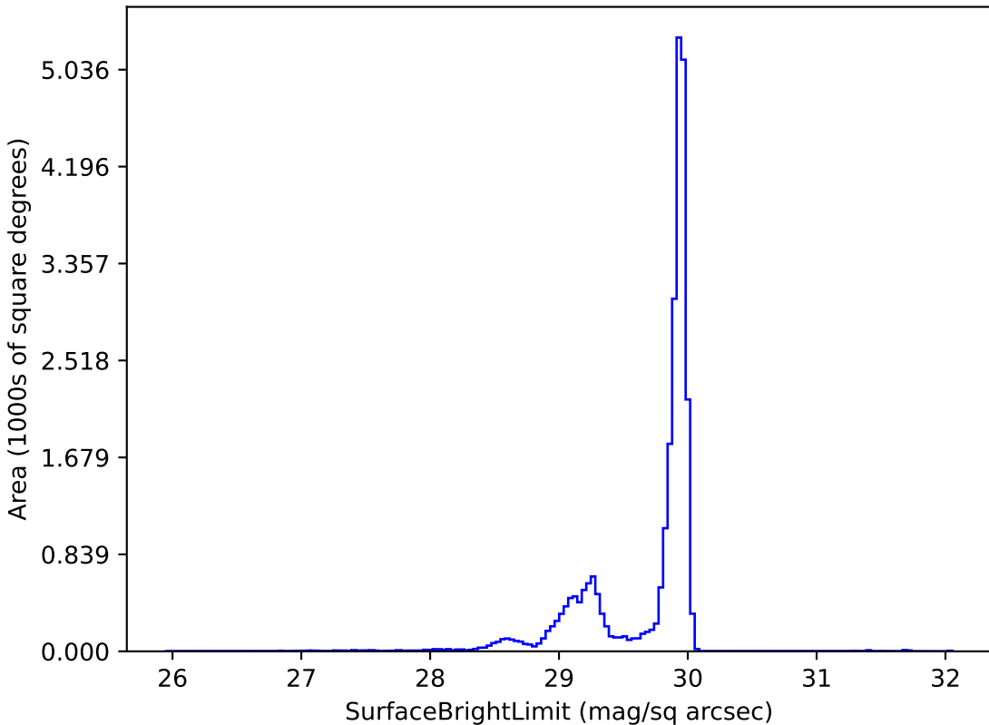
too_elab_r16_d2_gz_v3.4_10yrs i: SurfaceBrightLimit
