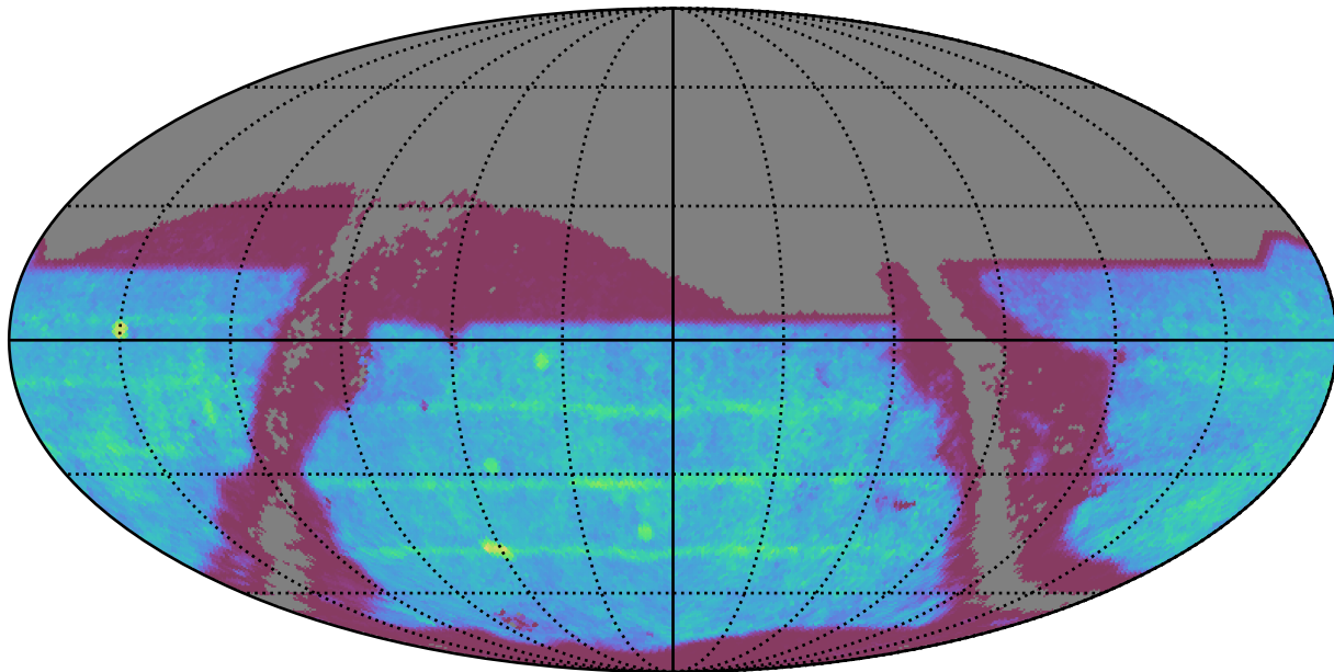
too_elab_r16_d2_gz_v3.4_10yrs : SNSLMetric
