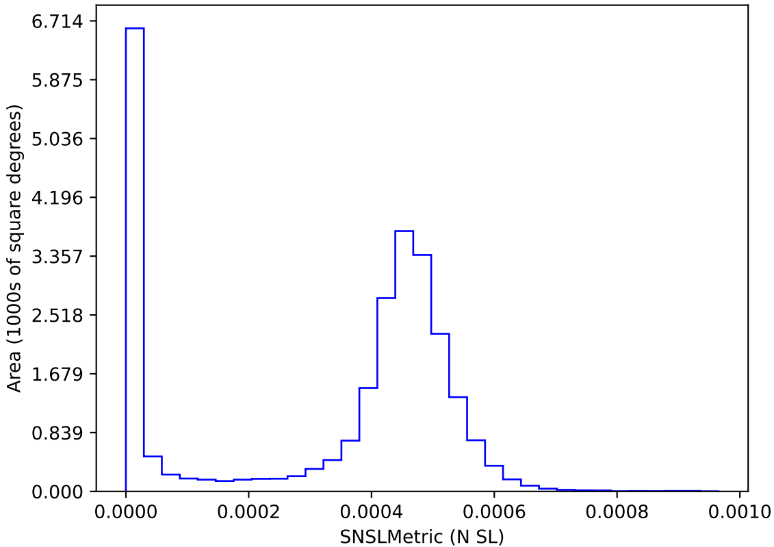
too_elab_r16_d2_gz_v3.4_10yrs : SNSLMetric
