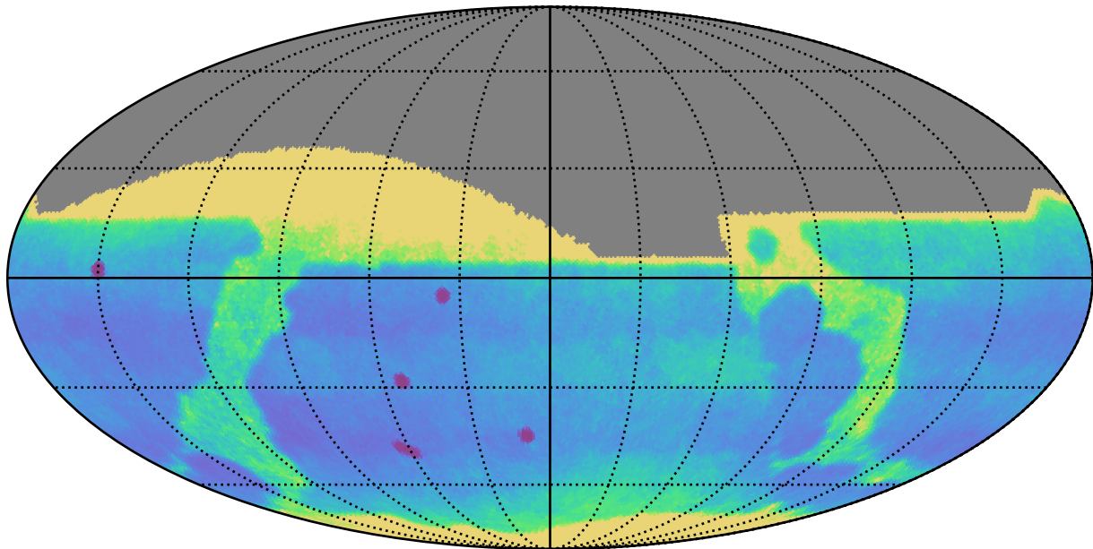
too_elab_r16_d2_gz_v3.4_10yrs : Proper Motion Uncert @ 24.0
