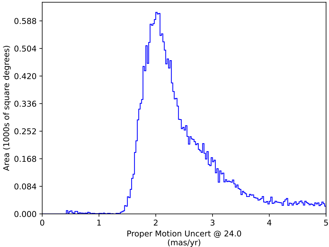
too_elab_r16_d2_gz_v3.4_10yrs : Proper Motion Uncert @ 24.0
