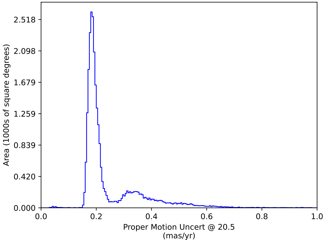
too_elab_r16_d2_gz_v3.4_10yrs : Proper Motion Uncert @ 20.5
