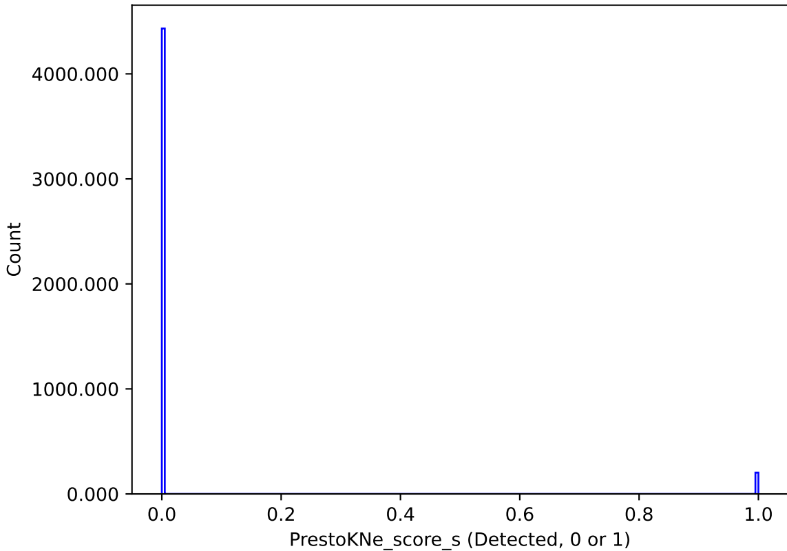
too_elab_r16_d2_gz_v3.4_10yrs : PrestoKNe_score_s
