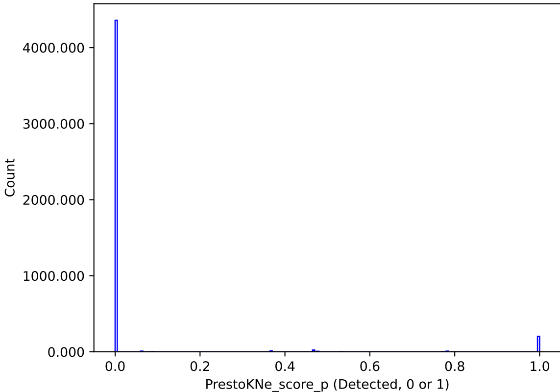
too_elab_r16_d2_gz_v3.4_10yrs : PrestoKNe_score_p
