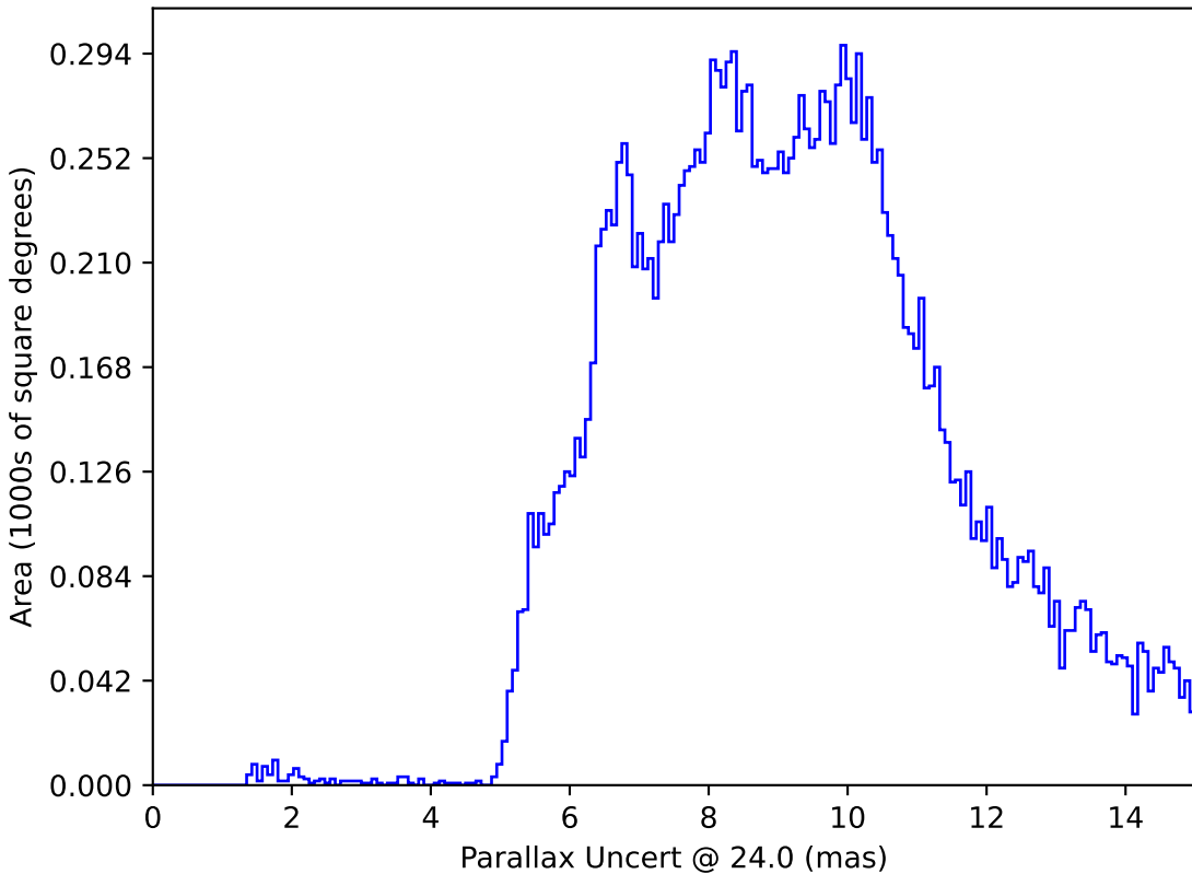
too_elab_r16_d2_gz_v3.4_10yrs : Parallax Uncert @ 24.0
