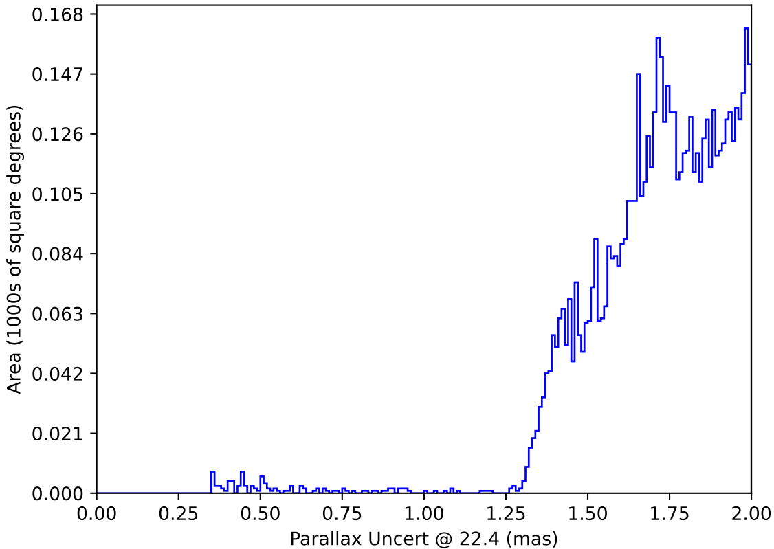
too_elab_r16_d2_gz_v3.4_10yrs : Parallax Uncert @ 22.4
