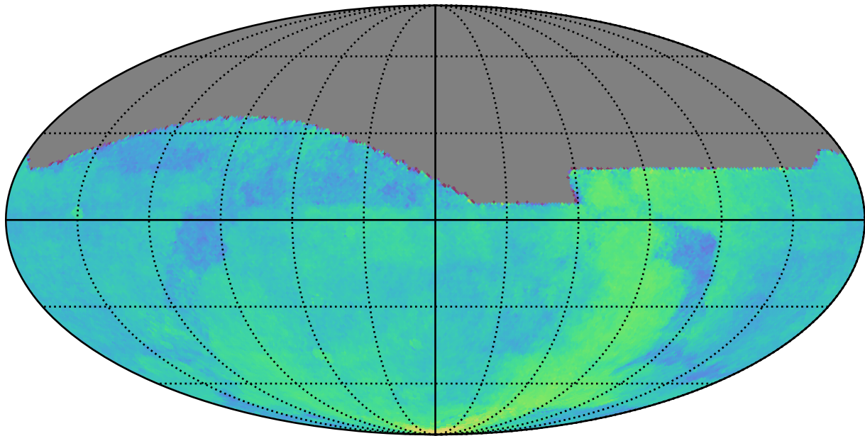
too_elab_r16_d2_gz_v3.4_10yrs : Parallax Coverage @ 24.0
