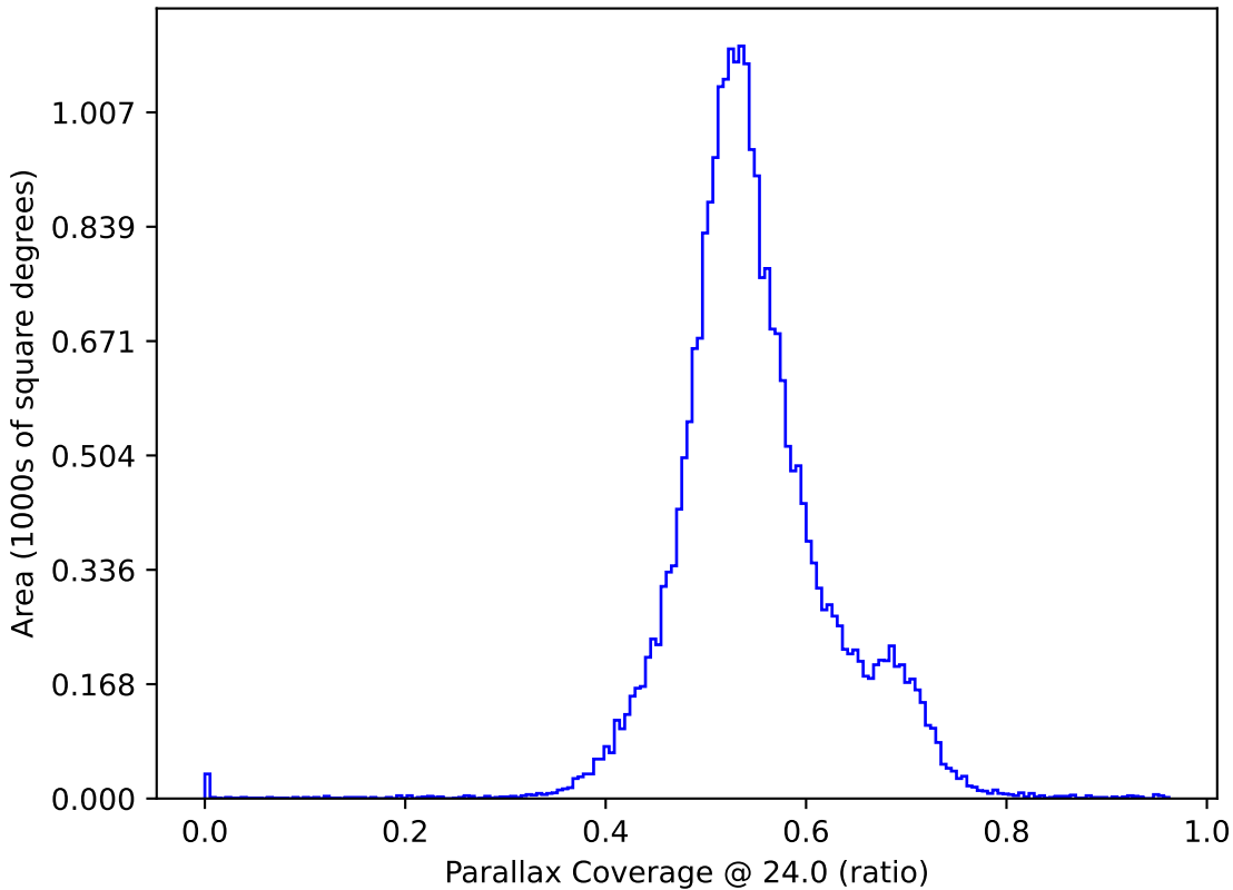
too_elab_r16_d2_gz_v3.4_10yrs : Parallax Coverage @ 24.0
