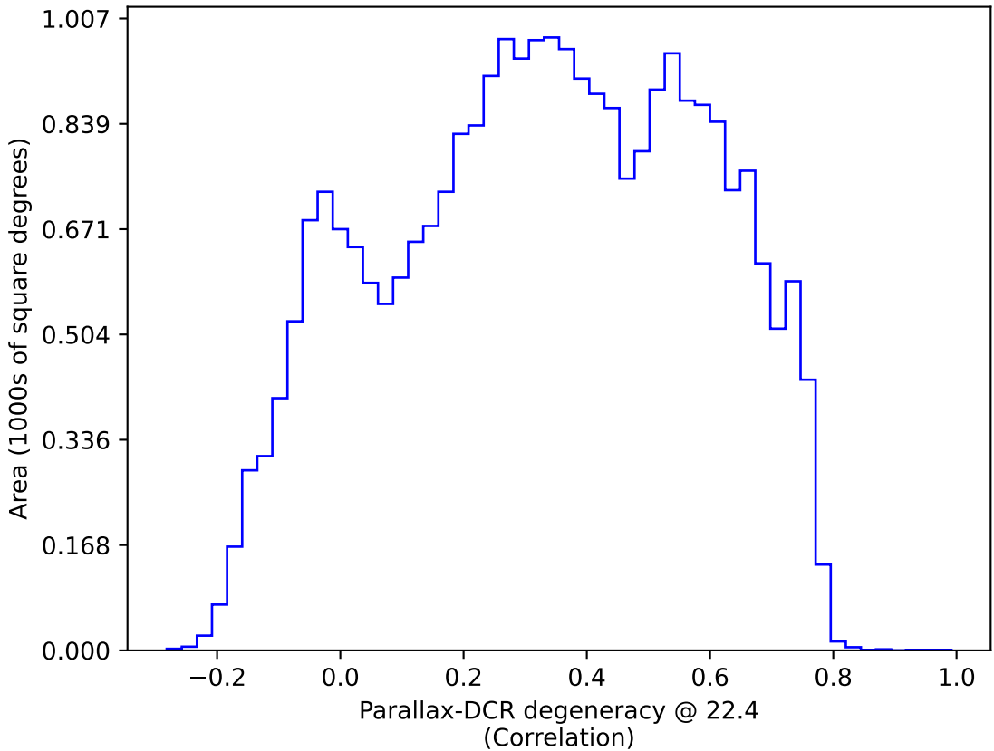
too_elab_r16_d2_gz_v3.4_10yrs : Parallax-DCR degeneracy @ 22.4
