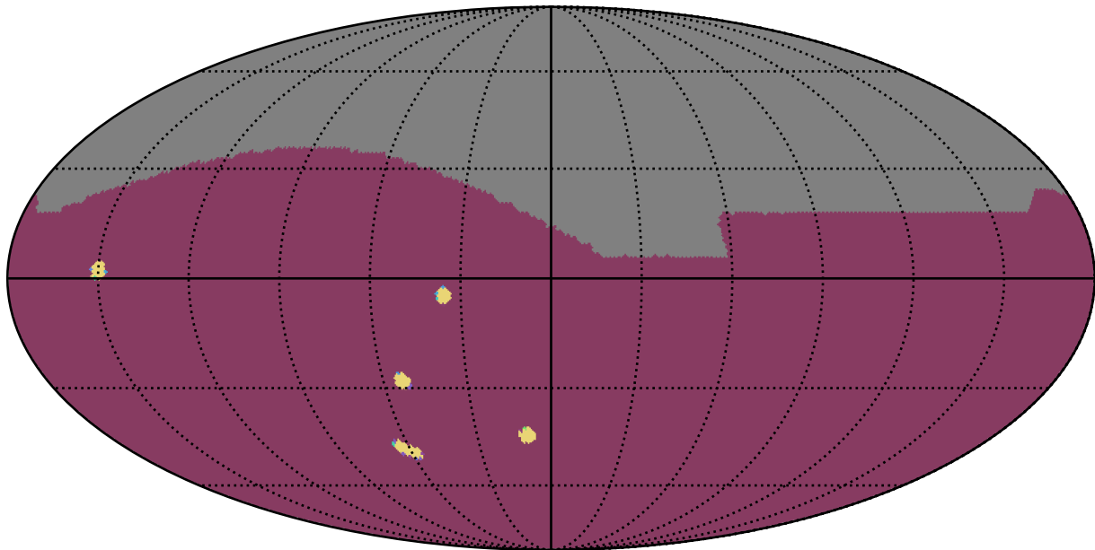
too_elab_r16_d2_gz_v3.4_10yrs : NumberOfQuickRevisits
