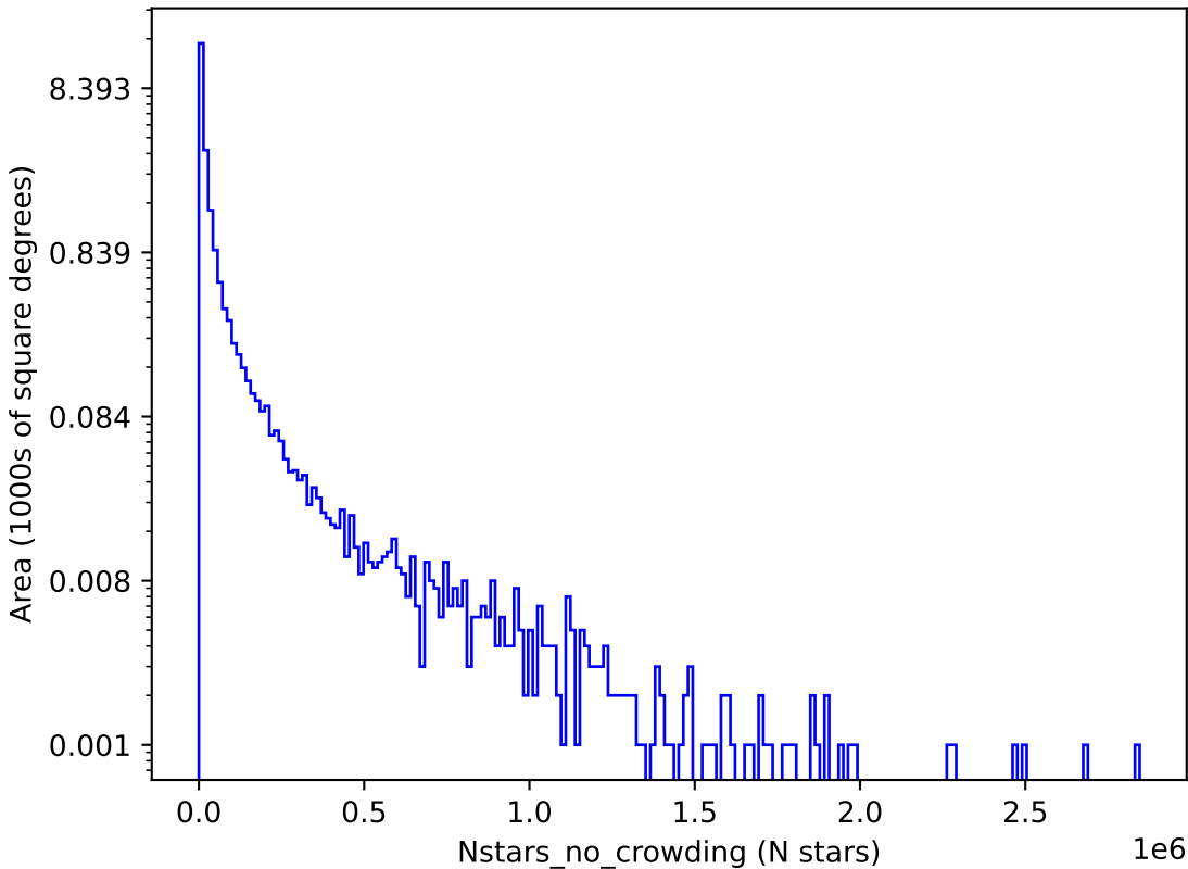
too_elab_r16_d2_gz_v3.4_10yrs u: Nstars_no_crowding
