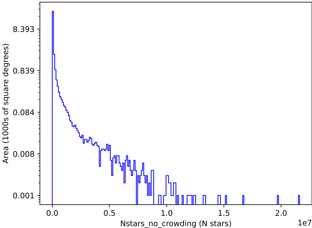
too_elab_r16_d2_gz_v3.4_10yrs r: Nstars_no_crowding
