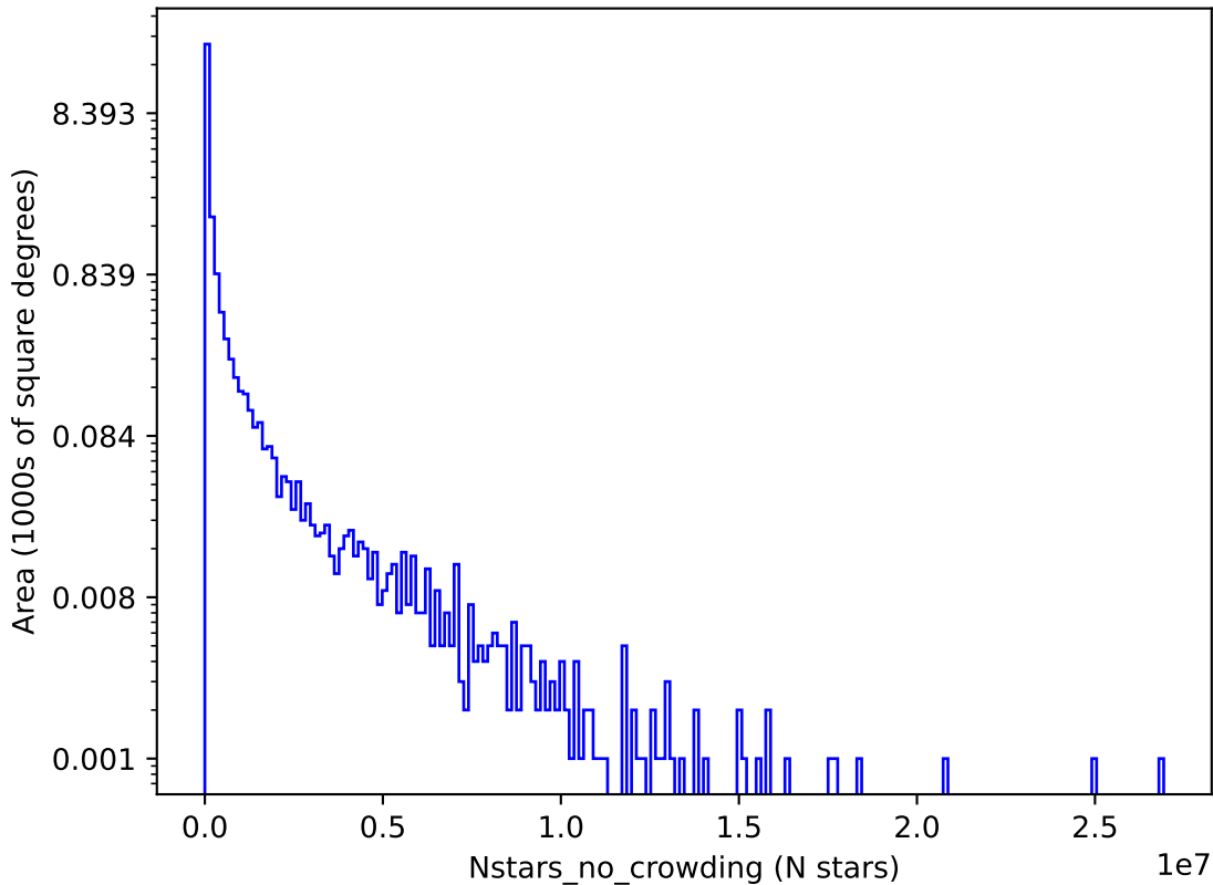
too_elab_r16_d2_gz_v3.4_10yrs i: Nstars_no_crowding
