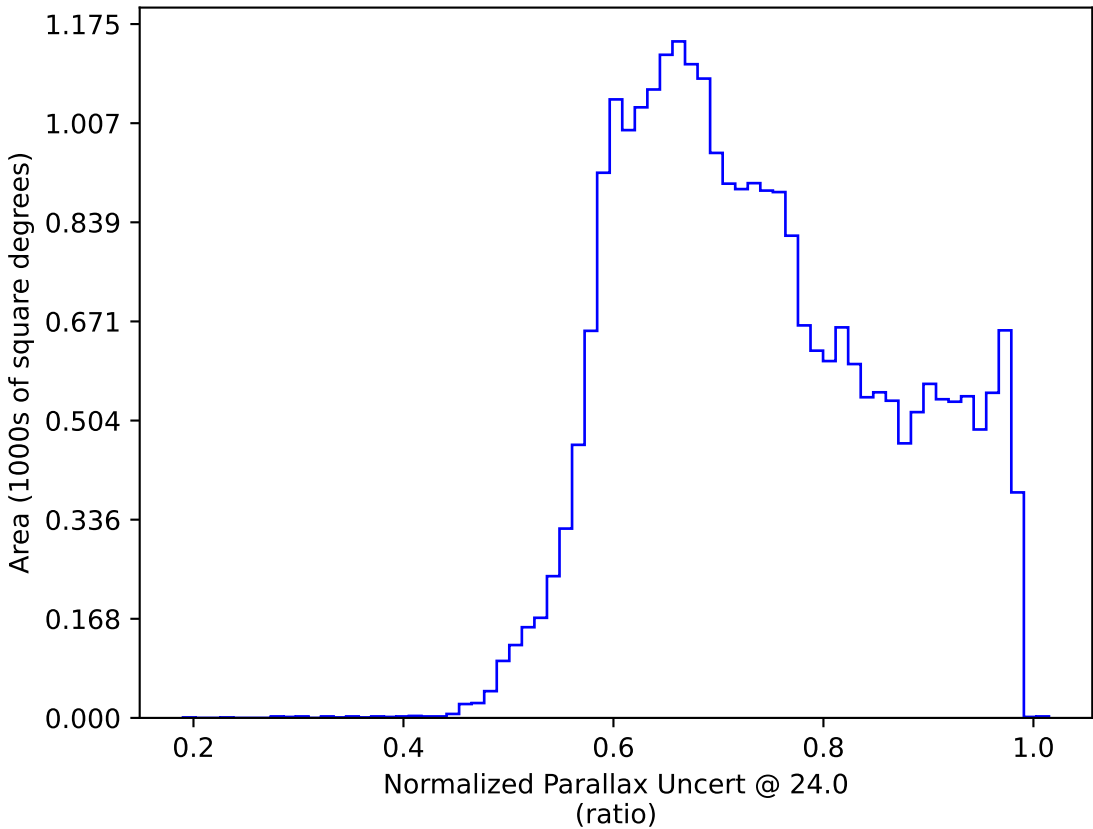
too_elab_r16_d2_gz_v3.4_10yrs : Normalized Parallax Uncert @ 24.0
