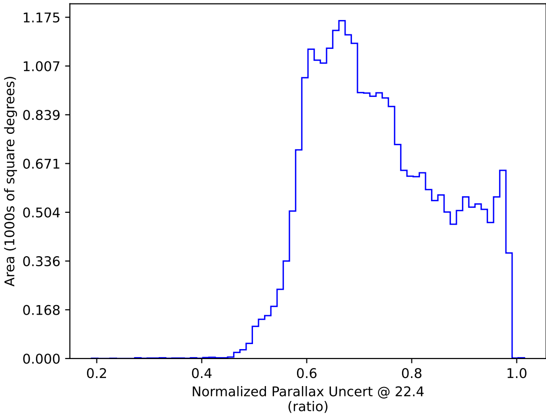
too_elab_r16_d2_gz_v3.4_10yrs : Normalized Parallax Uncert @ 22.4
