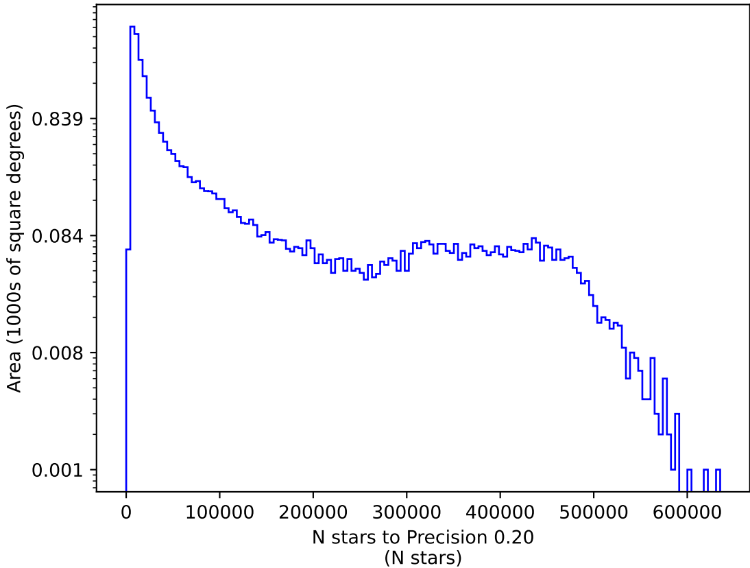
too_elab_r16_d2_gz_v3.4_10yrs r: N stars to Precision 0.20
