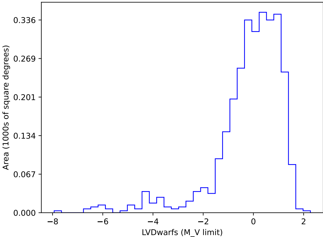
too_elab_r16_d2_gz_v3.4_10yrs gi SCP: LVDwarfs
