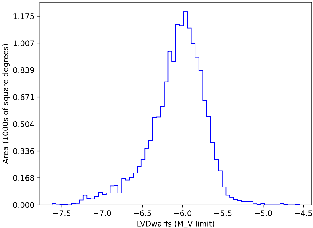
too_elab_r16_d2_gz_v3.4_10yrs gi: LVDwarfs
