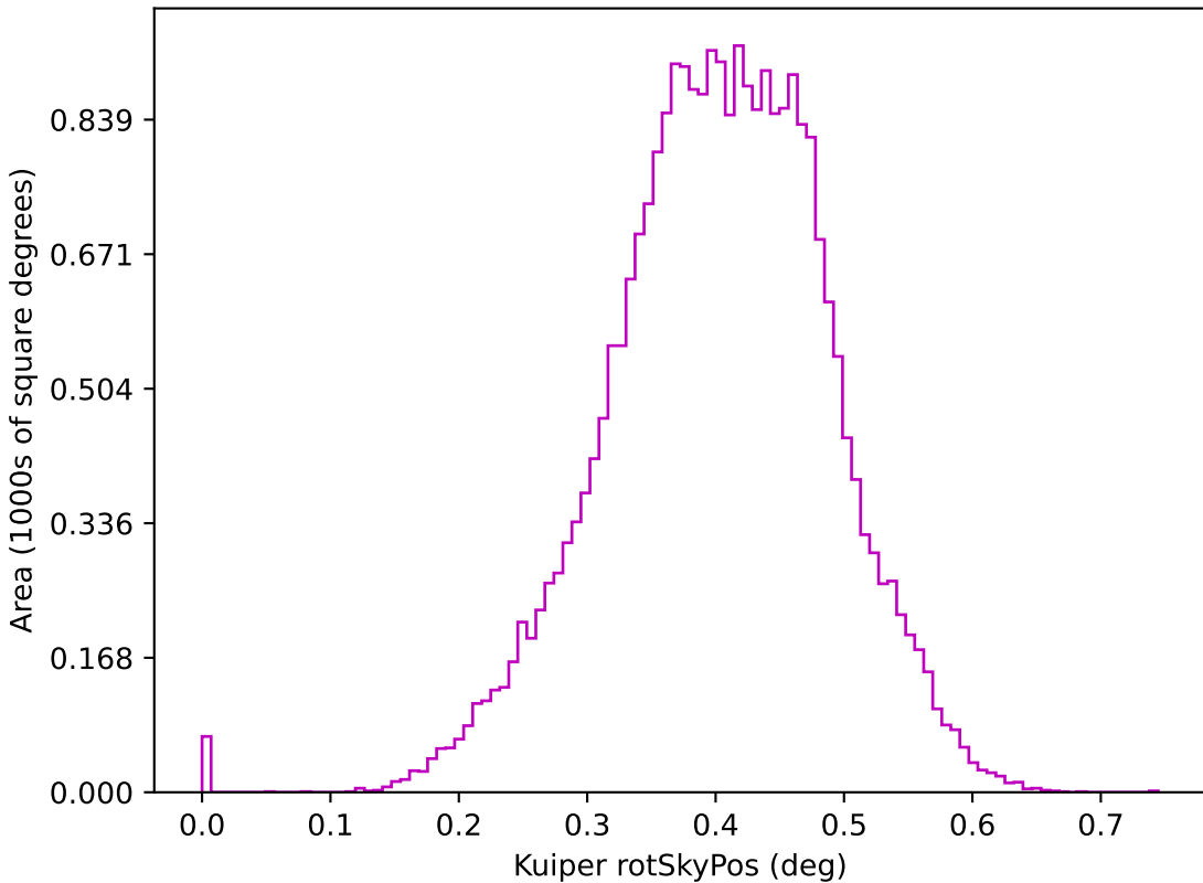
too_elab_r16_d2_gz_v3.4_10yrs z: Kuiper rotSkyPos
