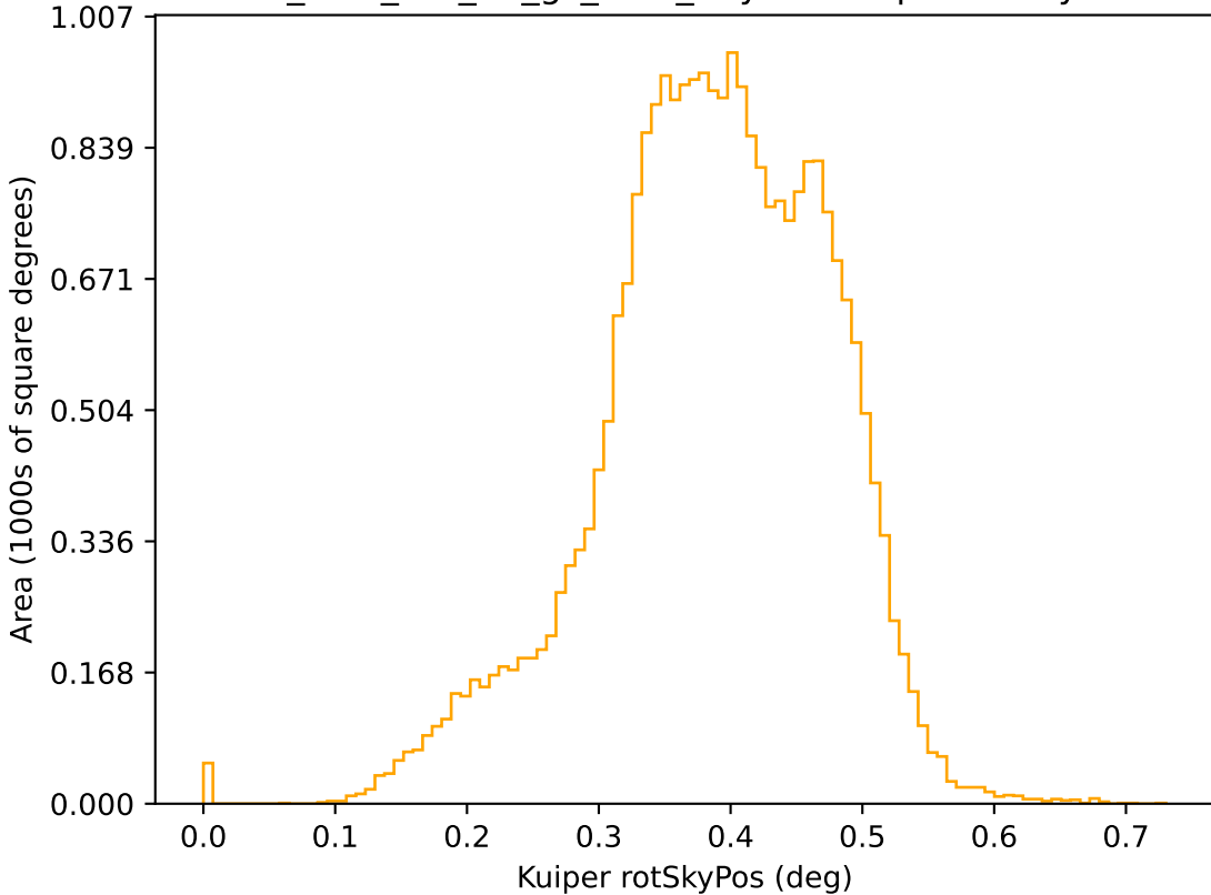
too_elab_r16_d2_gz_v3.4_10yrs r: Kuiper rotSkyPos
