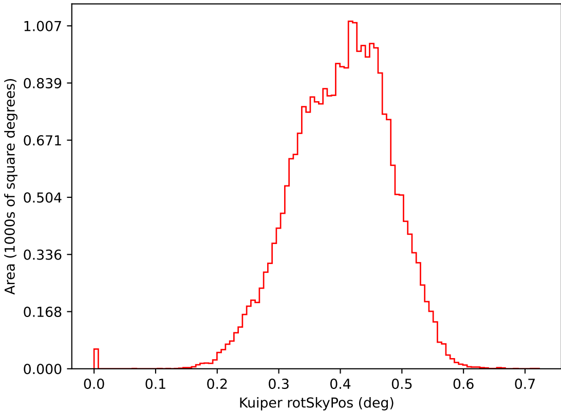
too_elab_r16_d2_gz_v3.4_10yrs i: Kuiper rotSkyPos
