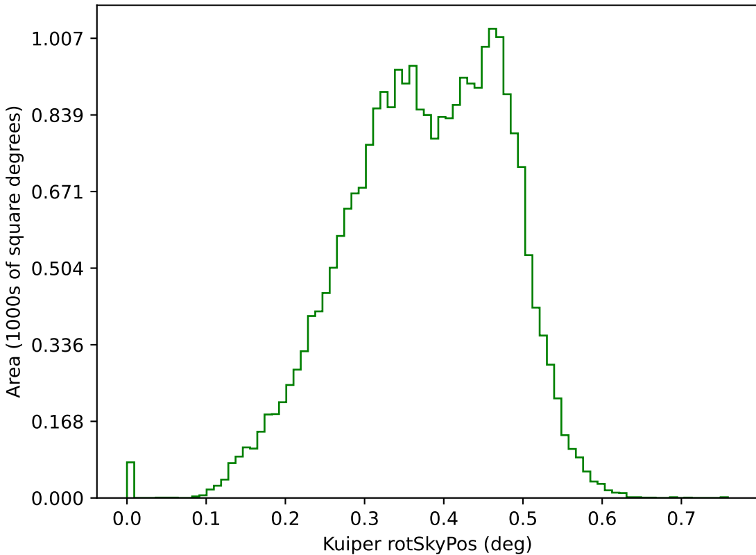
too_elab_r16_d2_gz_v3.4_10yrs g: Kuiper rotSkyPos
