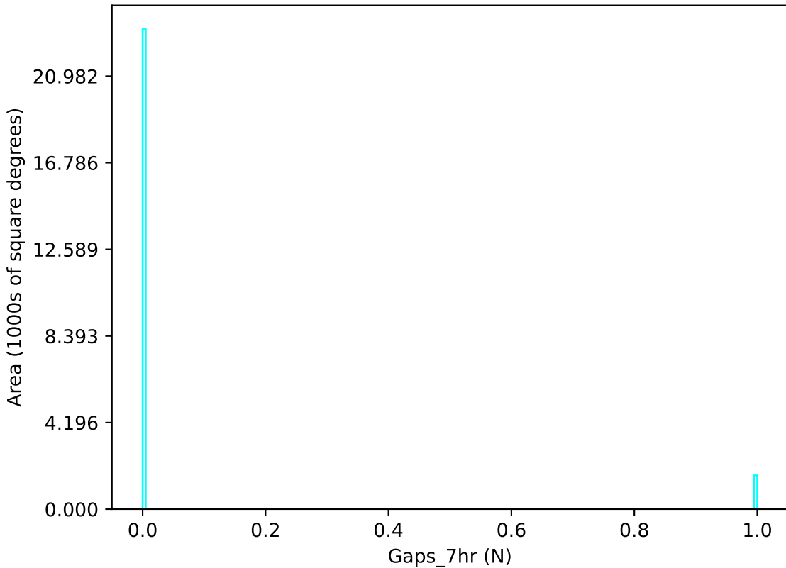
too_elab_r16_d2_gz_v3.4_10yrs u band: Gaps_7hr
