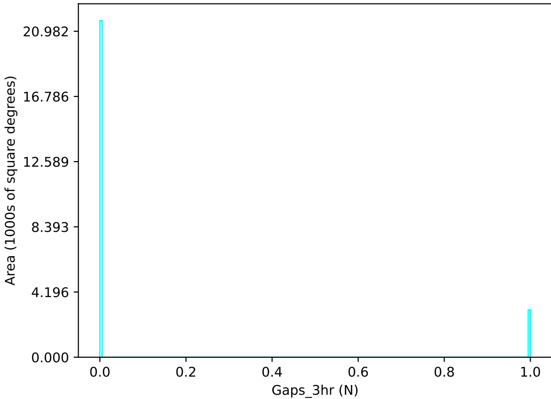
too_elab_r16_d2_gz_v3.4_10yrs u band: Gaps_3hr
