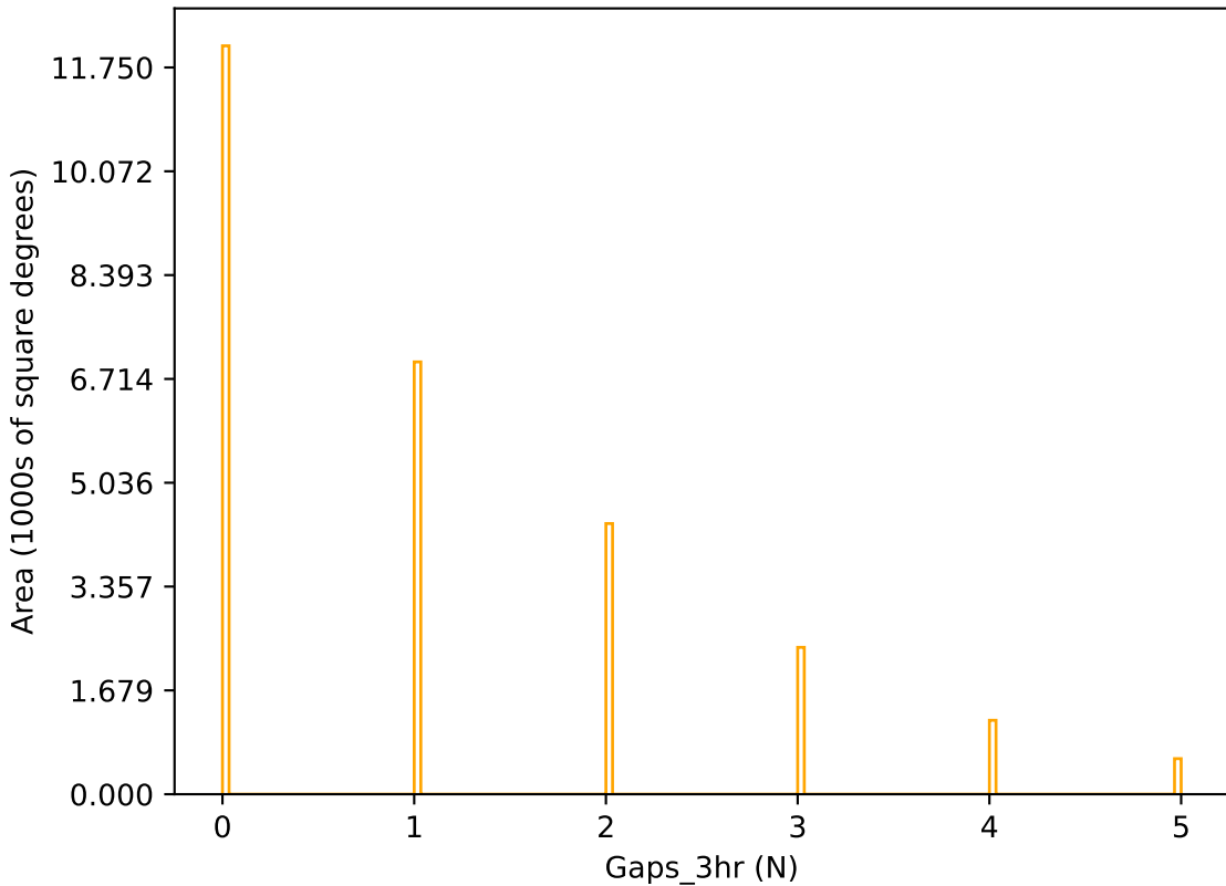
too_elab_r16_d2_gz_v3.4_10yrs r band: Gaps_3hr
