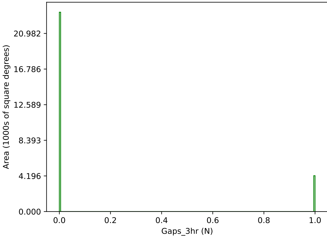
too_elab_r16_d2_gz_v3.4_10yrs g band: Gaps_3hr
