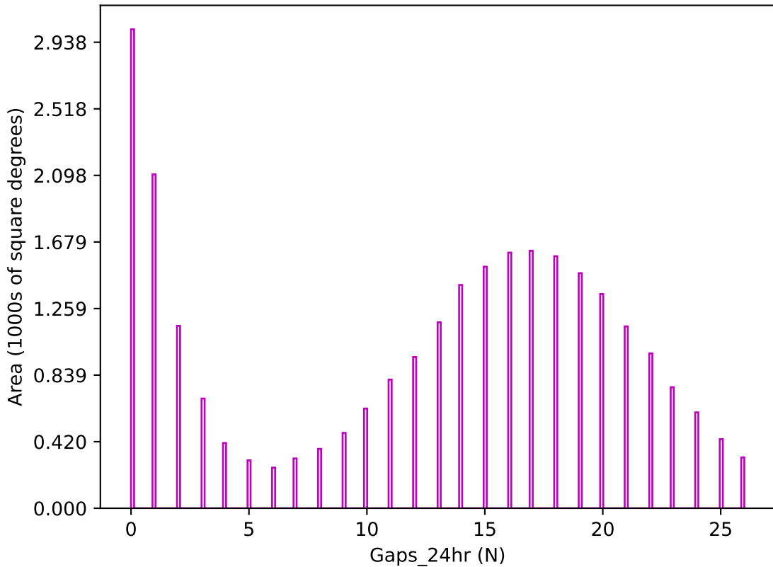
too_elab_r16_d2_gz_v3.4_10yrs z band: Gaps_24hr
