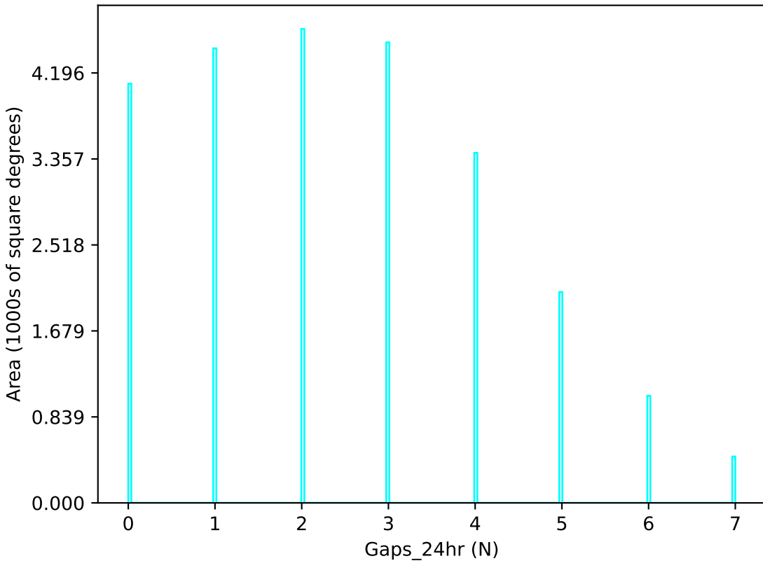
too_elab_r16_d2_gz_v3.4_10yrs u band: Gaps_24hr
