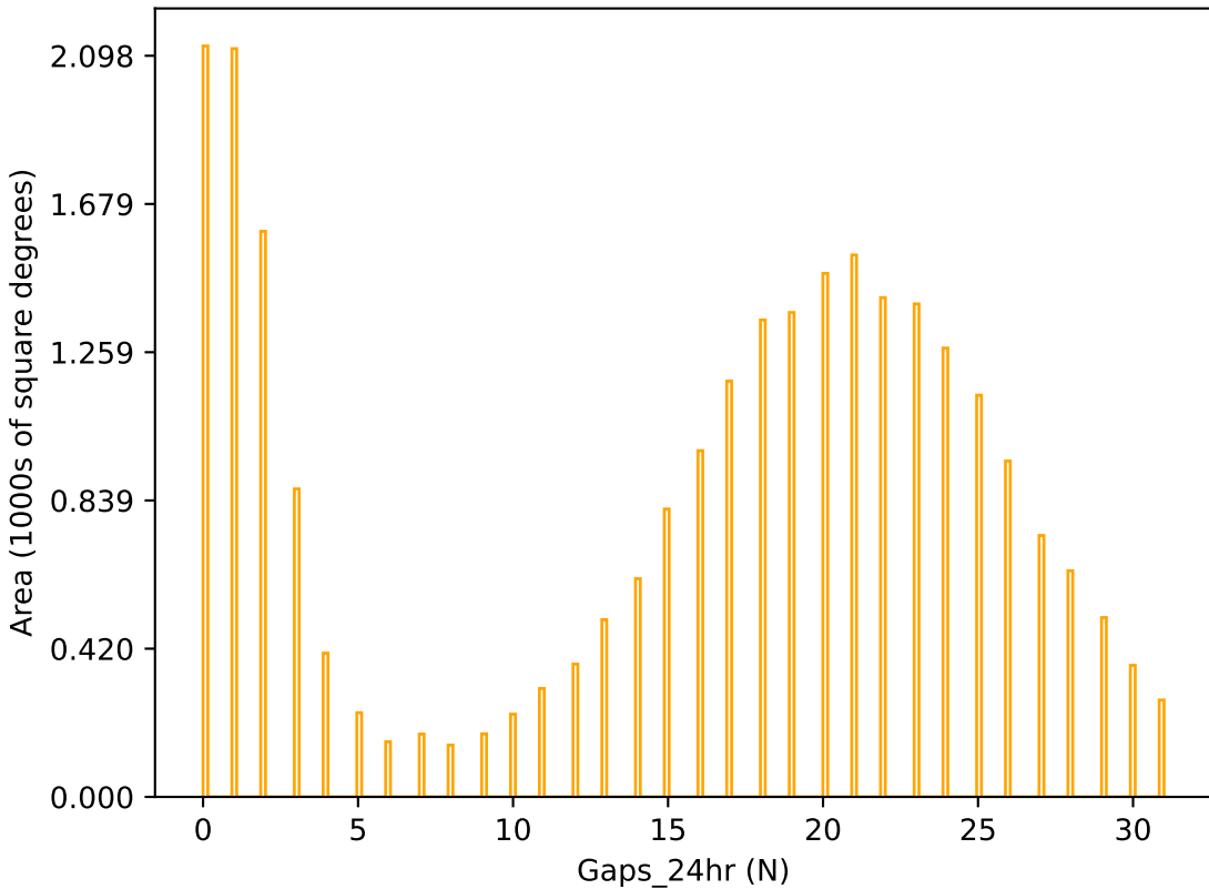
too_elab_r16_d2_gz_v3.4_10yrs r band: Gaps_24hr
