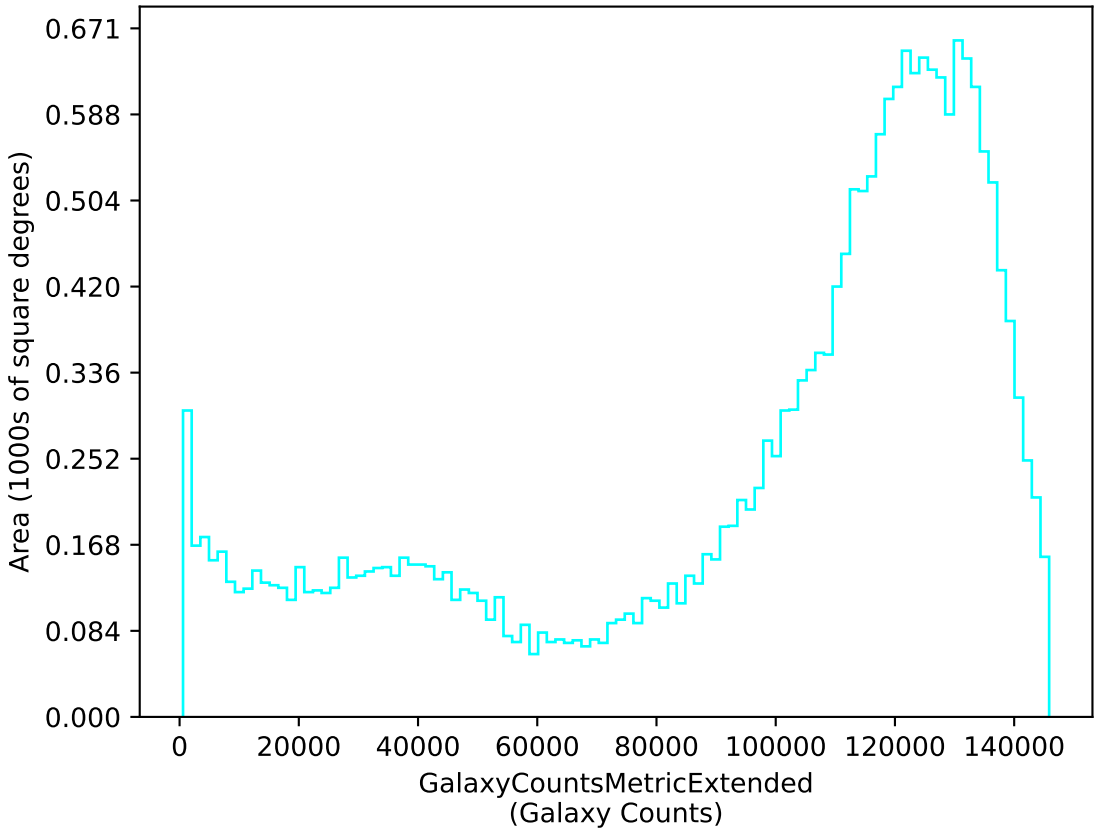
too_elab_r16_d2_gz_v3.4_10yrs u: GalaxyCountsMetricExtended
