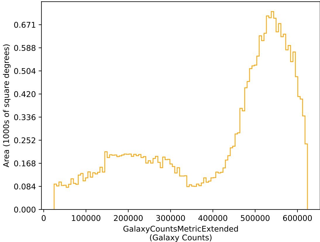
too_elab_r16_d2_gz_v3.4_10yrs r: GalaxyCountsMetricExtended
