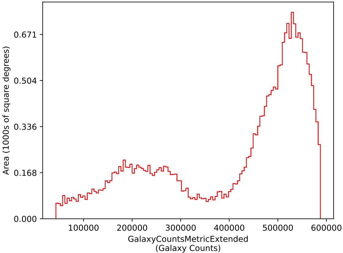
too_elab_r16_d2_gz_v3.4_10yrs i: GalaxyCountsMetricExtended
