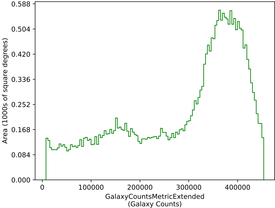
too_elab_r16_d2_gz_v3.4_10yrs g: GalaxyCountsMetricExtended
