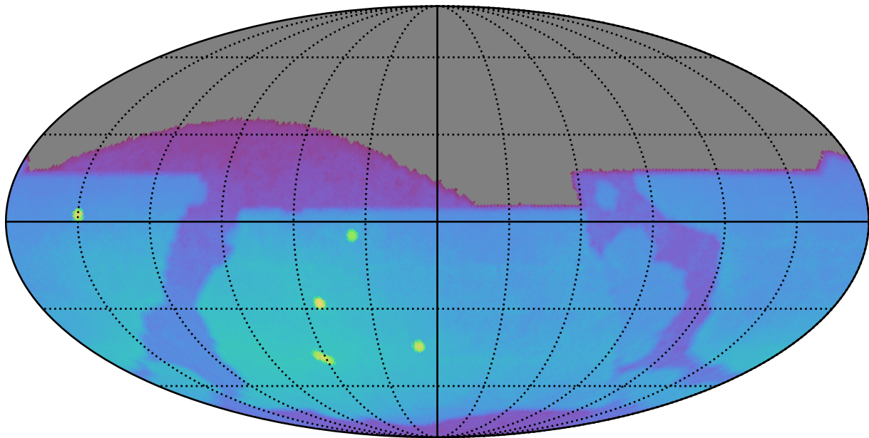
too_elab_r16_d2_gz_v3.4_10yrs : Brown Dwarf, L7
