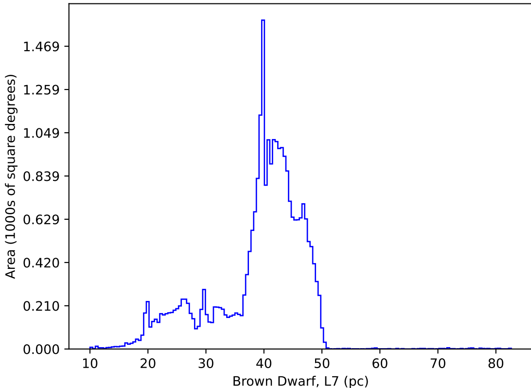
too_elab_r16_d2_gz_v3.4_10yrs : Brown Dwarf, L7
