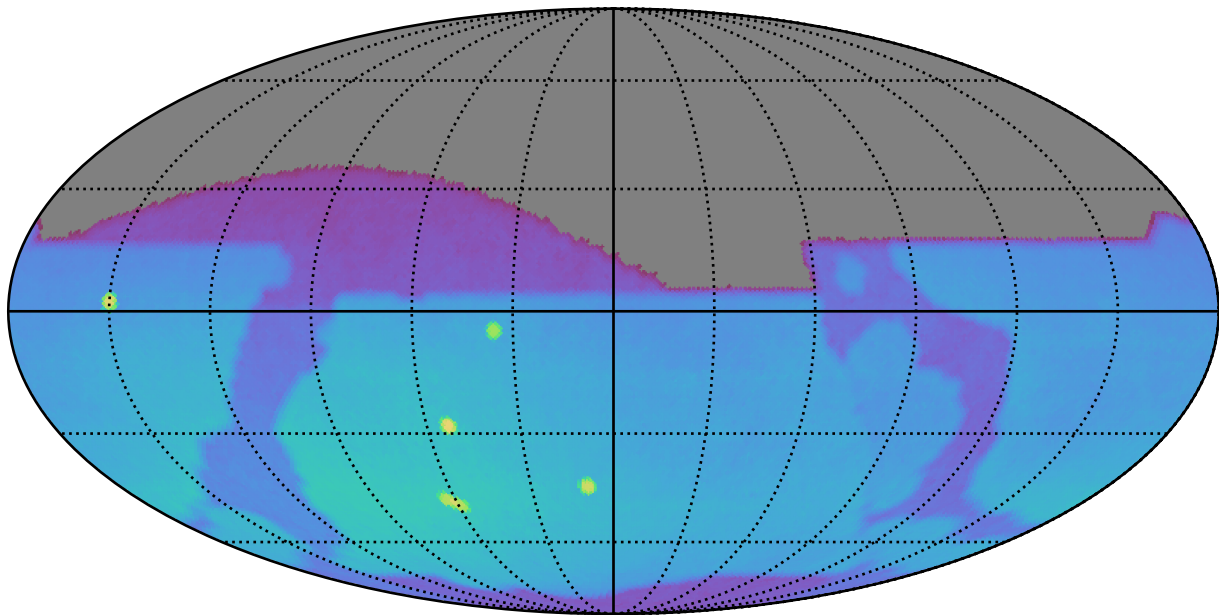
too_elab_r16_d2_gz_v3.4_10yrs : Brown Dwarf, L4
